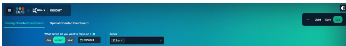
Figure 31 – Background settings
